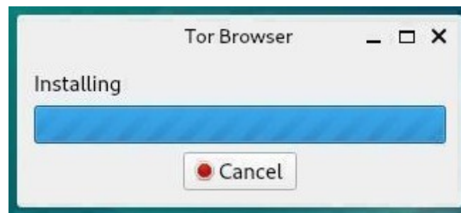
TorBrowser: Installation
